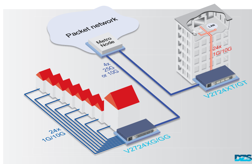
Typical applications with V2724XG/GG and V2724XT/GT
