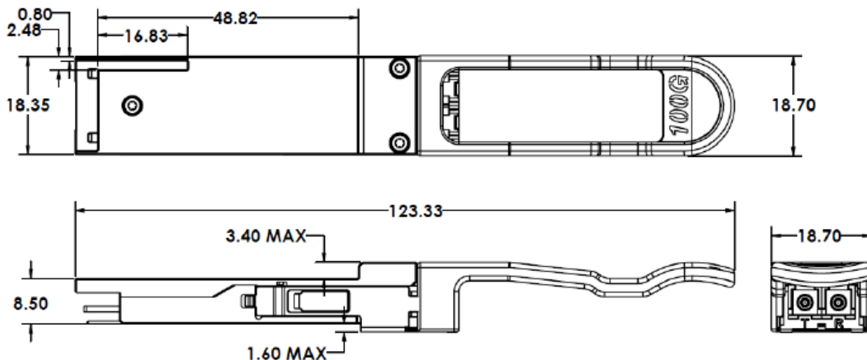
Figure 2. FTLC1152RGPL Mechanical Dimensions.
