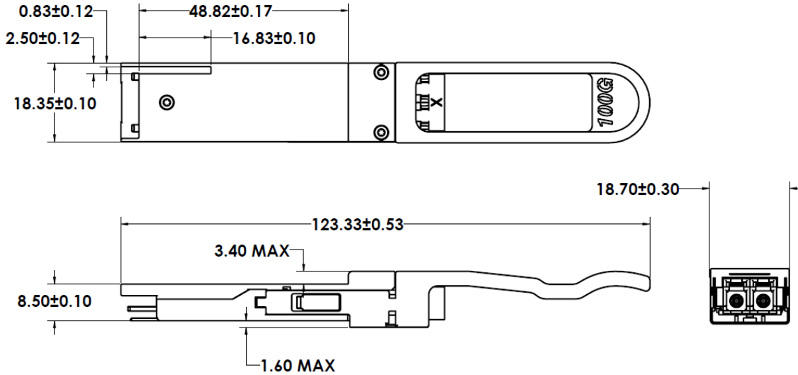
Figure 2. FTLC1155RGPLD Mechanical Dimensions.
