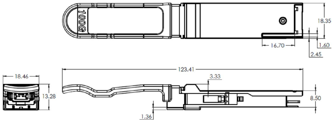
Figure 2. FTLC9555QEPM Mechanical Dimensions.
