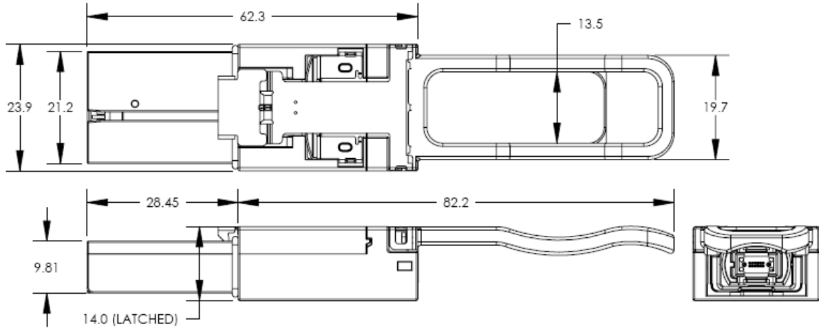
Figure 3 – FTLD12CL3C mechanical drawing
