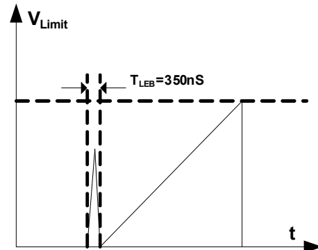
Figure 6: Leading-Edge Blanking
