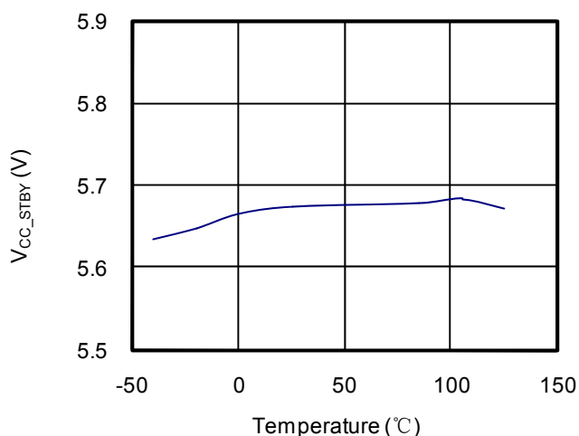
V_{\text{CCSTBY}} vs. Temperature
