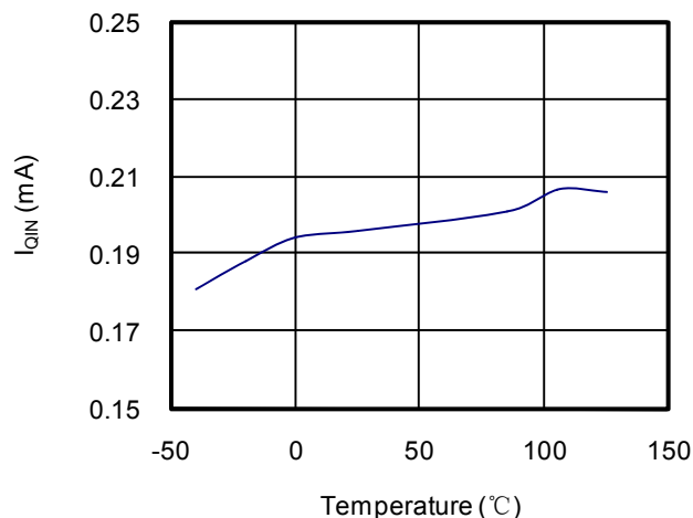
I_{QIN} @ V_{IN} = 5.5V vs. Temperature
