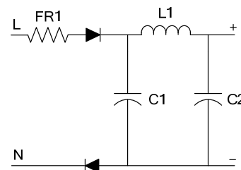
Figure 6: Half-Wave Rectifier
