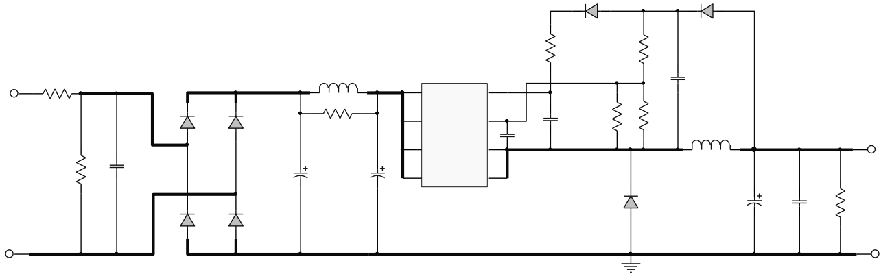
Figure 10: Typical Application at 12V, 300mA
