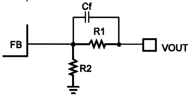
Figure 5: Feedback Network
