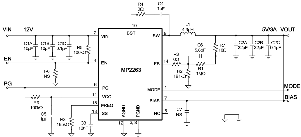
Figure 7: V_{IN} = 12V , V_{OUT} = 5V
