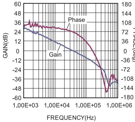
Loop Gain vs. Frequency V_{IN}=4.2V , I_{OUT}=1.5A
