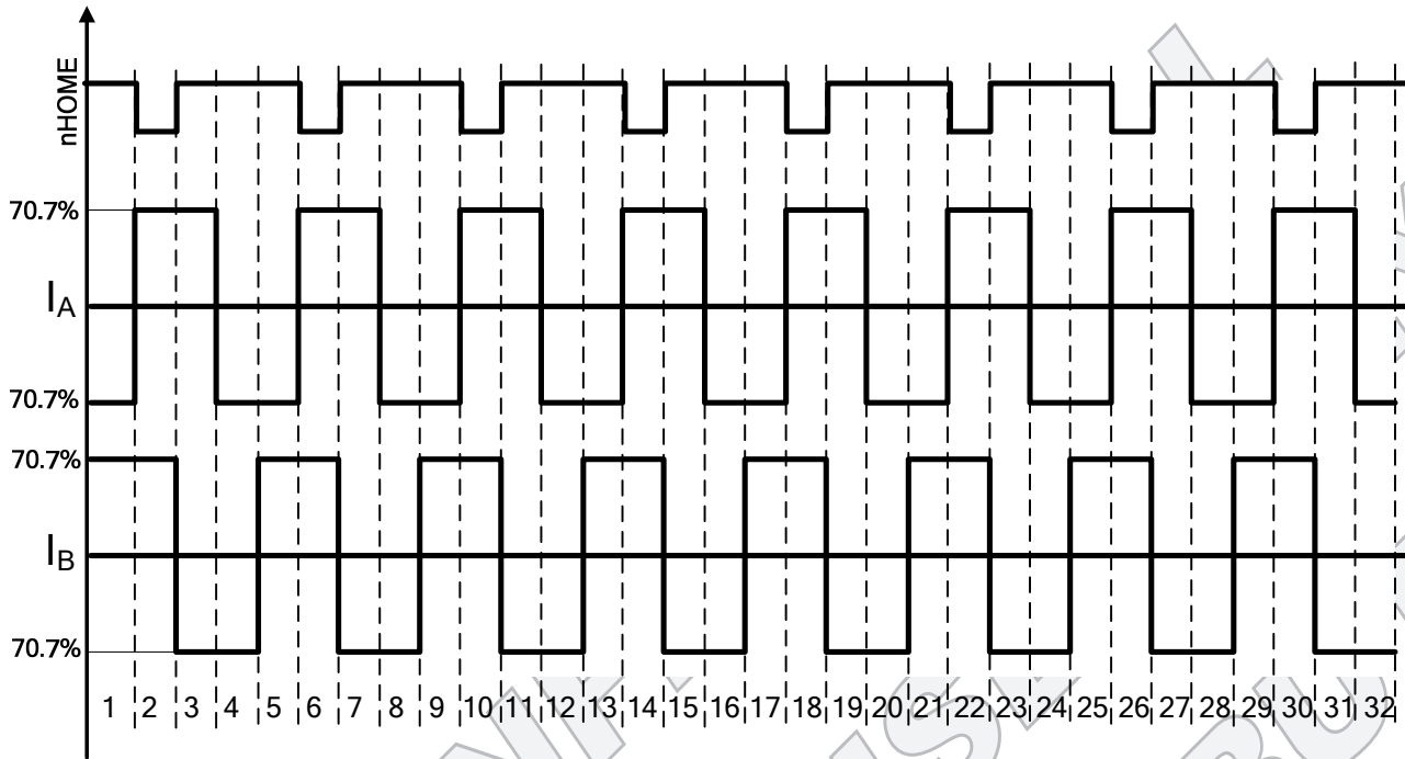
Figure 3a: Full Step (4 Step Sequences)
