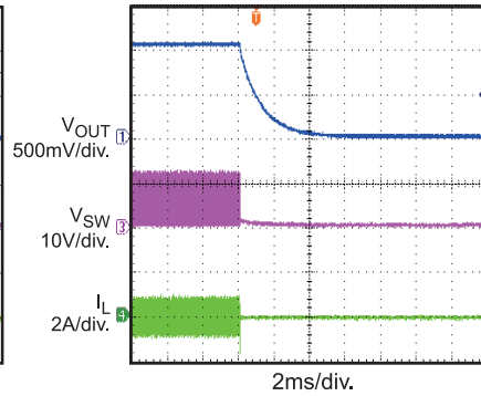
Thermal Shutdown
