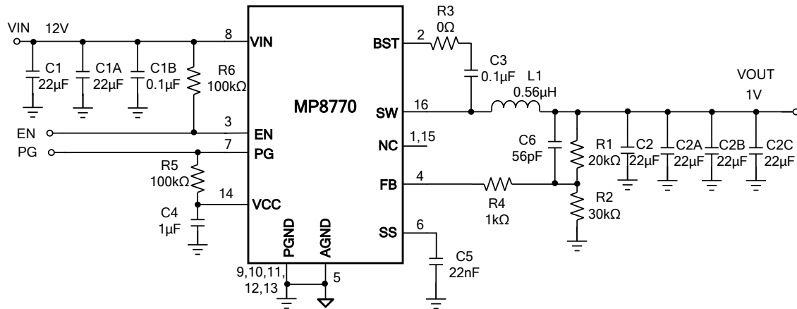
Figure 9: V_{IN} = 12V , V_{OUT} = 1V , I_{OUT} = 8A^{(7)}
