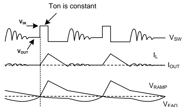
Figure 4: Light-Load Operation
