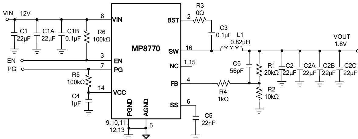
Figure 12: VIN = 12V, VOUT = 1.8V, IOUT = 8A (7)
