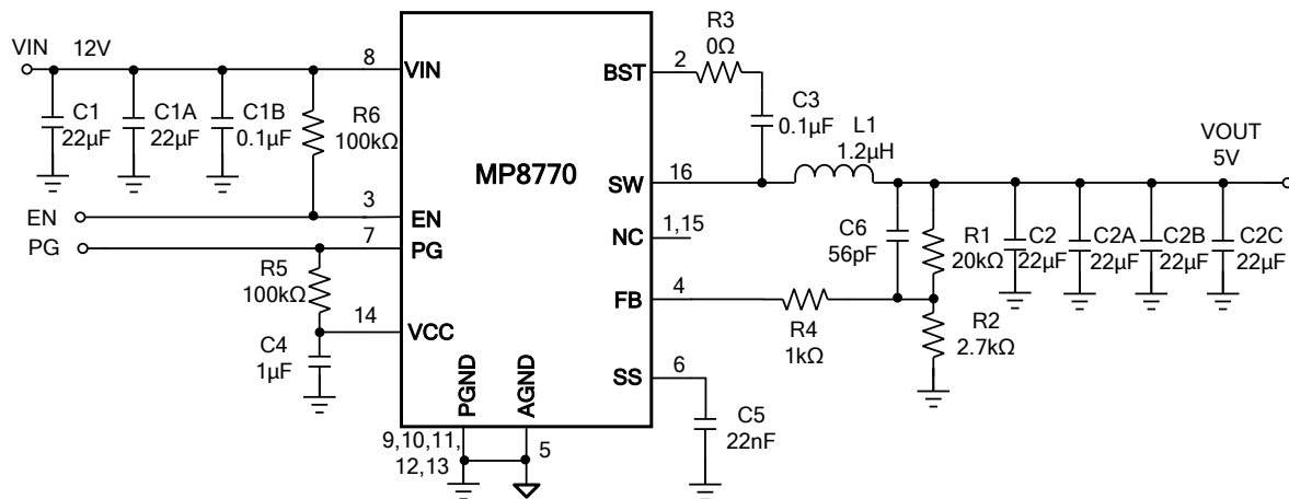
Figure 15: V_{IN} = 12V , V_{OUT} = 5V , I_{OUT} = 8A^{(7)}
