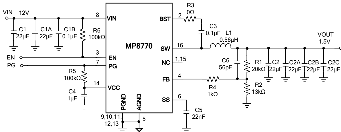
Figure 11: V_{IN} = 12V , V_{OUT} = 1.5V , I_{OUT} = 8A^{(7)}
