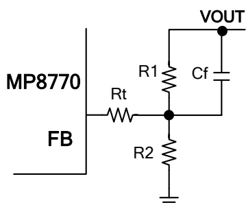
Figure 7: Feedback Network
