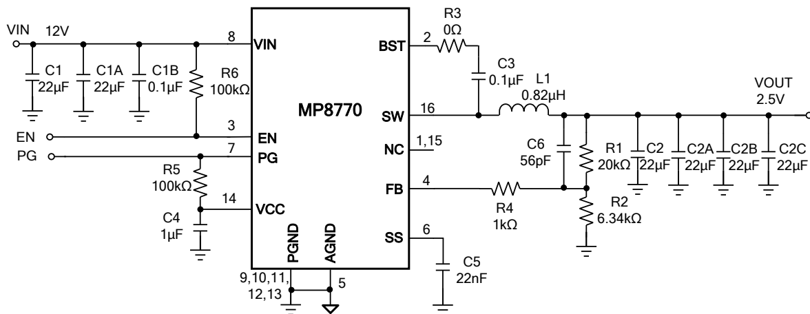
Figure 13: VIN = 12V, VOUT = 2.5V, IOUT = 8A (7)
