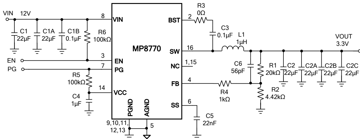
Figure 14: VIN = 12V, VOUT = 3.3V, IOUT = 8A (7)
