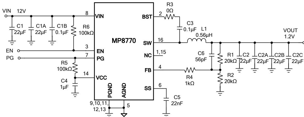
Figure 10: V_{IN} = 12V , V_{OUT} = 1.2V , I_{OUT} = 8A^{(7)}
