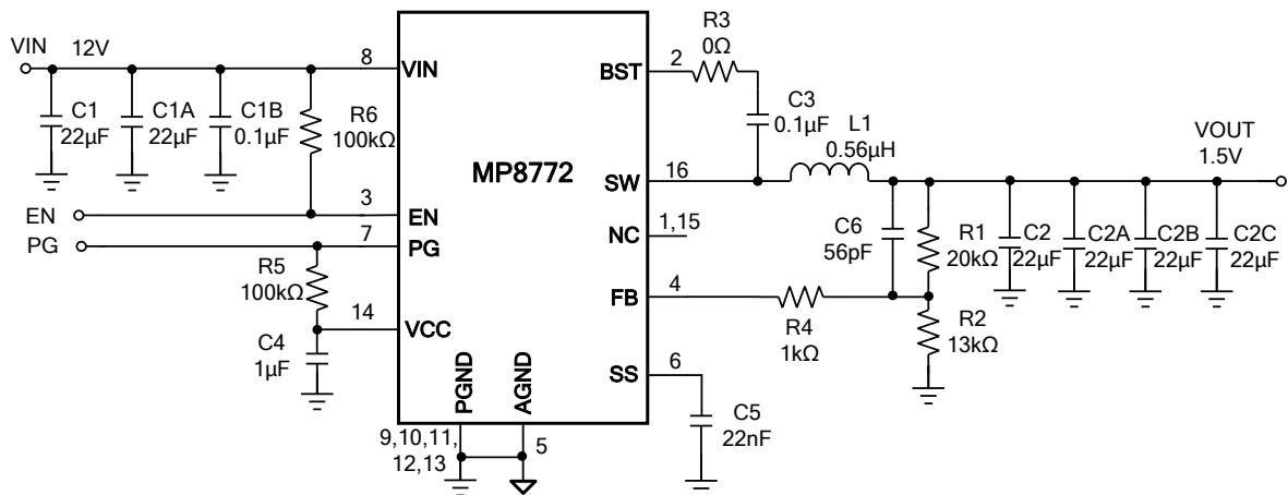
Figure 11: V_{IN} = 12V , V_{OUT} = 1.5V , I_{OUT} = 12A (7)
