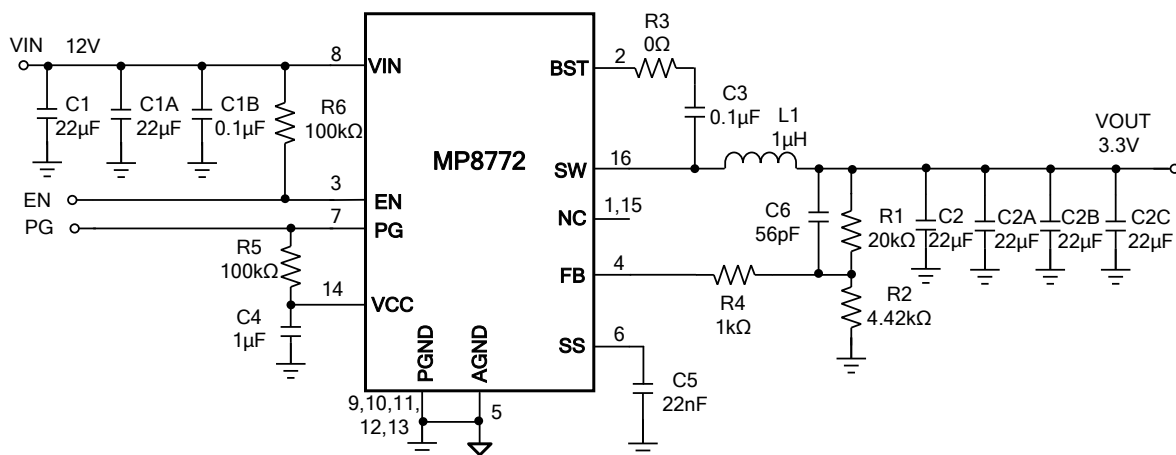
Figure 14: V_{IN} = 12V , V_{OUT} = 3.3V , I_{OUT} = 12A (7)
