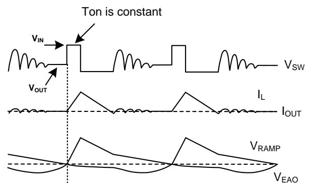
Figure 4: Light-Load Operation
