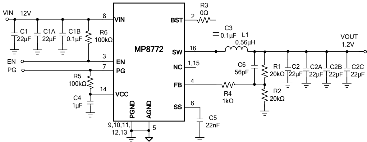
Figure 10: V_{IN} = 12V , V_{OUT} = 1.2V , I_{OUT} = 12A (7)
