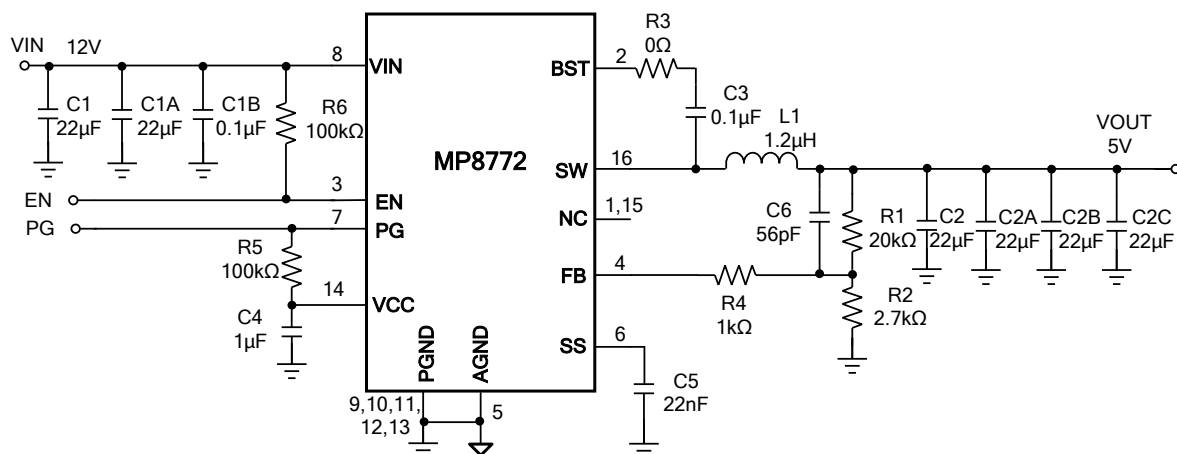
Figure 15: V_{IN} = 12V , V_{OUT} = 5V , I_{OUT} = 12A (7)
