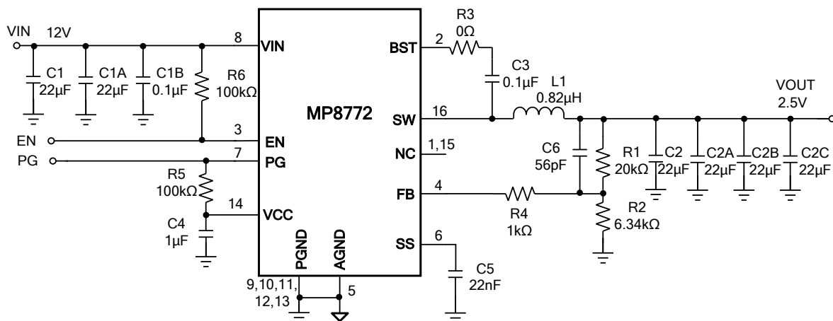
Figure 13: V_{IN} = 12V , V_{OUT} = 2.5V , I_{OUT} = 12A (7)
