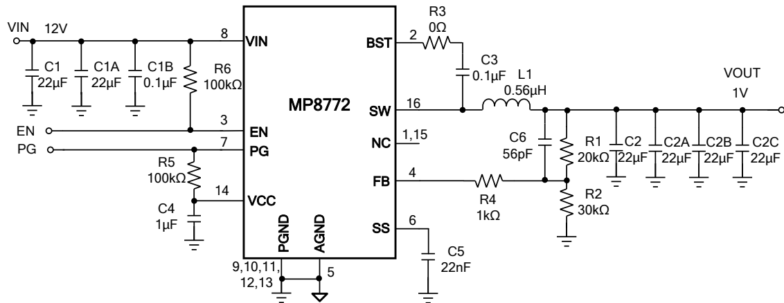
Figure 9: V_{IN} = 12V , V_{OUT} = 1V , I_{OUT} = 12A (7)
