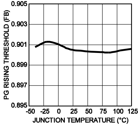
PG Rising Threshold vs. Junction Temperature VIN=24V
