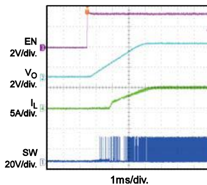
Start-up Through EN I_O = 5A
