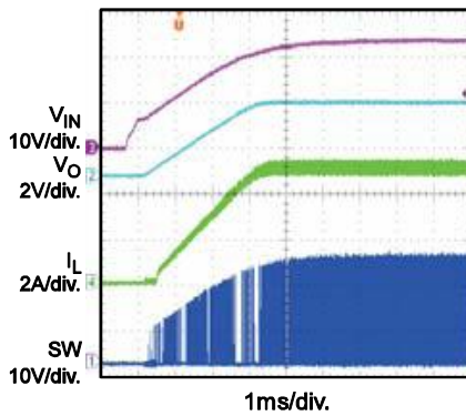
Start-up Through EN I_O = 0A
