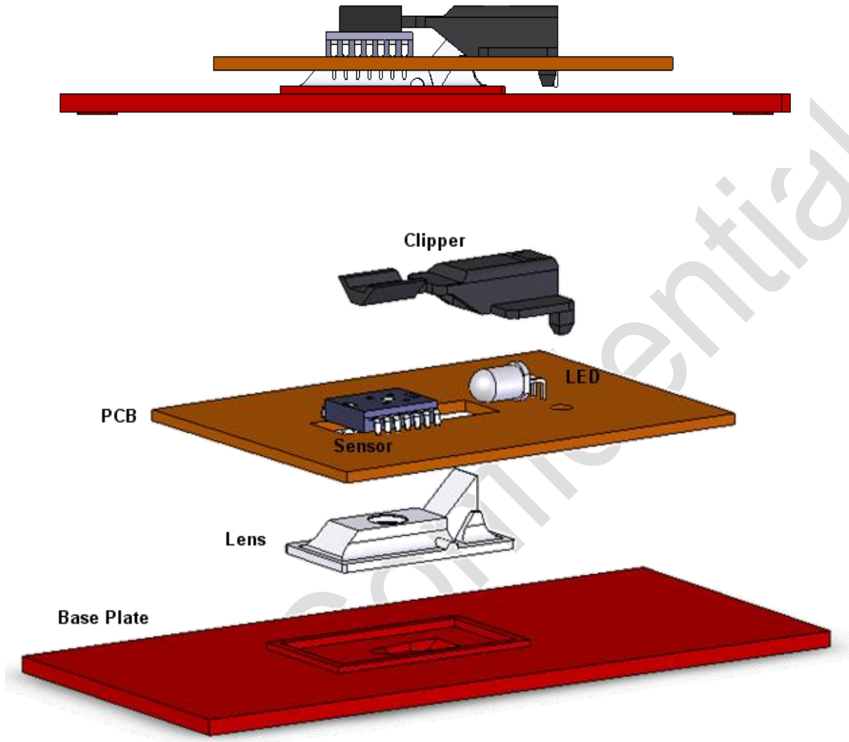
Figure 7. 3D Assembly for Mounting Instructions
