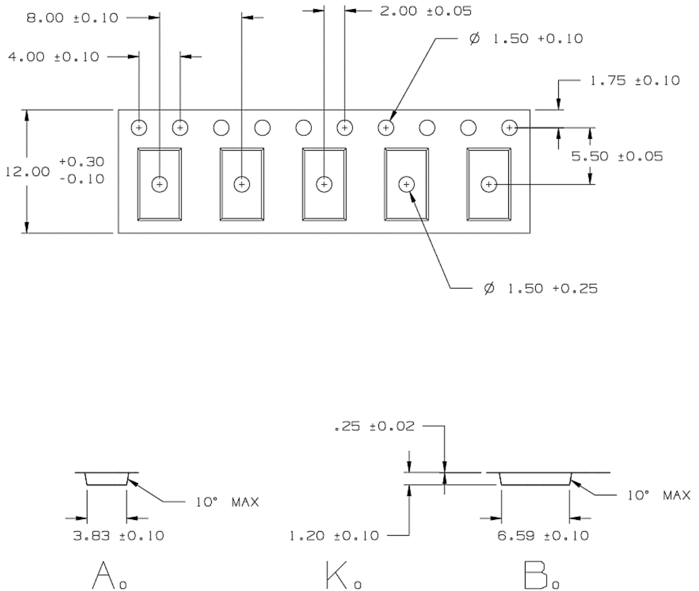
Figure 11. Carrier Drawing
